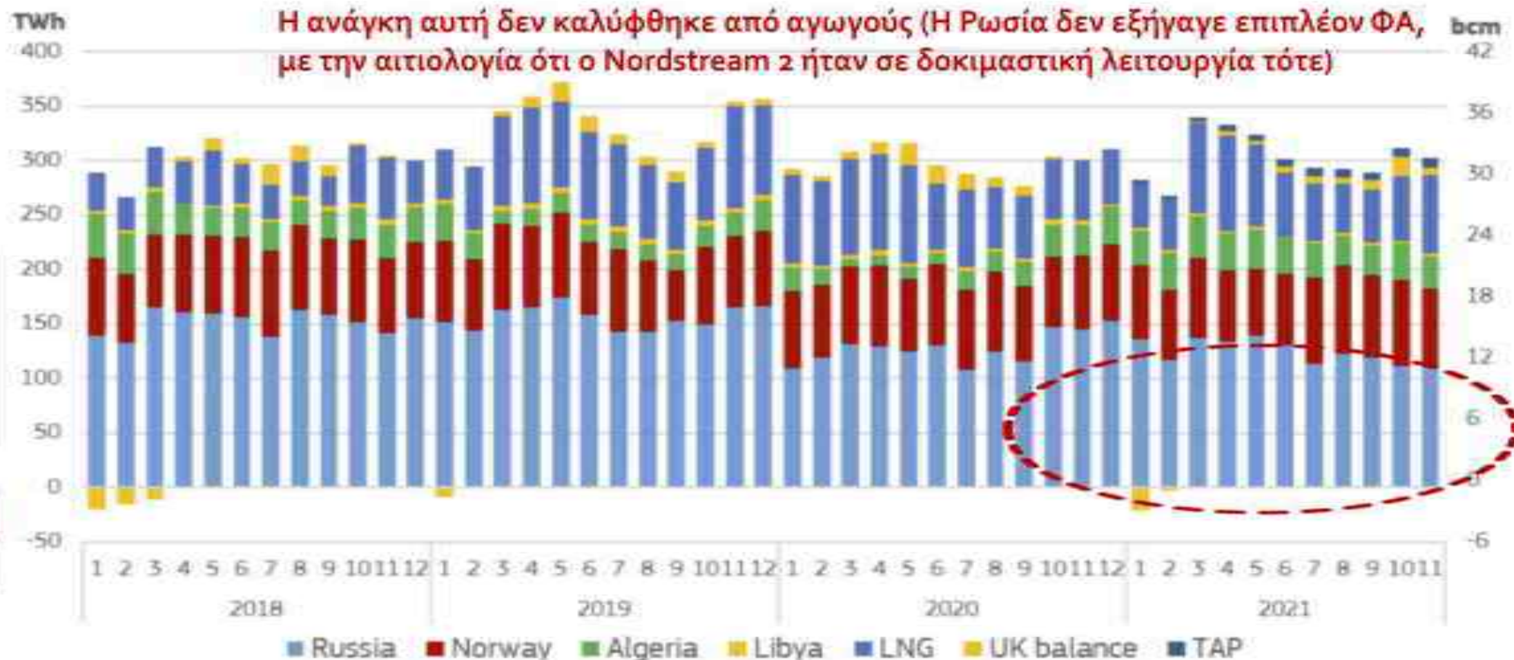
Figure 44 – Monthly evolution of gas imports from extra-EU sources
